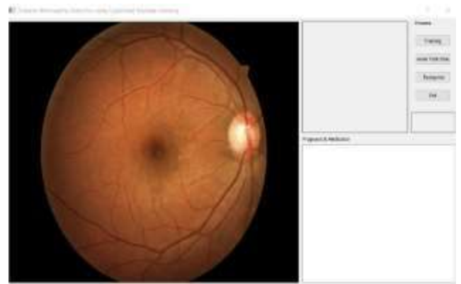
Fig. 4: Backend System
